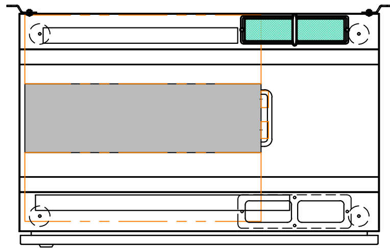
SECTION A-A ENCLOSURE BASE, LOOKING DOWN SCALE 1:7.5
