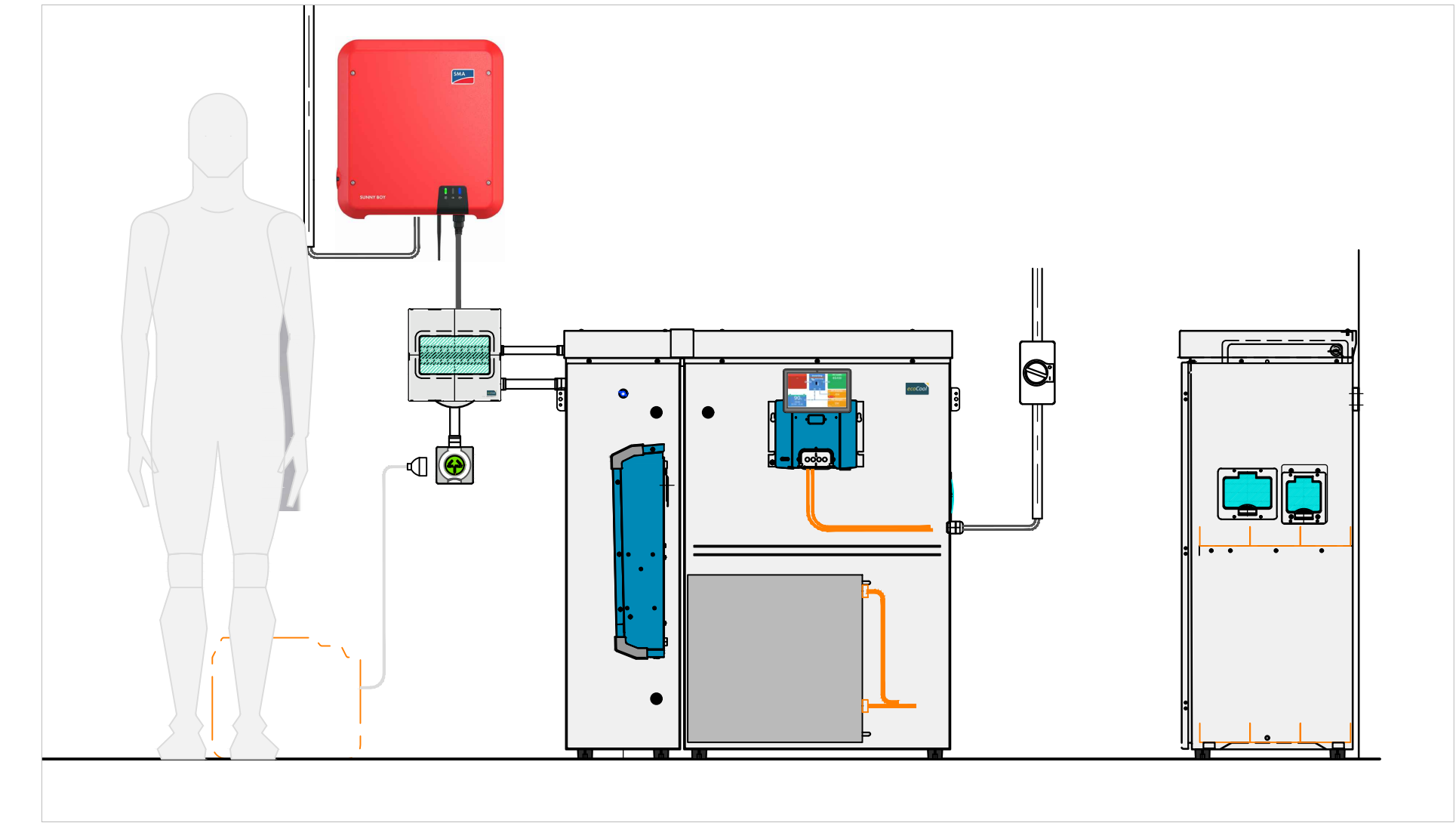
USE CASE: VICTRON SYSTEM FRONT VIEW SCALE 1:10
